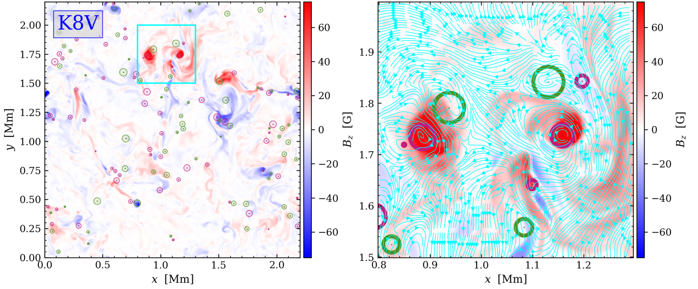
Fig. B.2. Vertical magnetic field, B_z , for the K8V stellar model during the saturation phase of the SSD in the high photosphere ( z = 183 km). Clockwise and counterclockwise vortices identified by the SWIRL algorithm in the horizontal plane are indicated by pink and green disks, respectively. The blue square in the left panel marks the boundaries of the zoomed region shown in the right panel, where the horizontal component of the velocity field at z = 183 km is represented by blue instantaneous streamlines.
