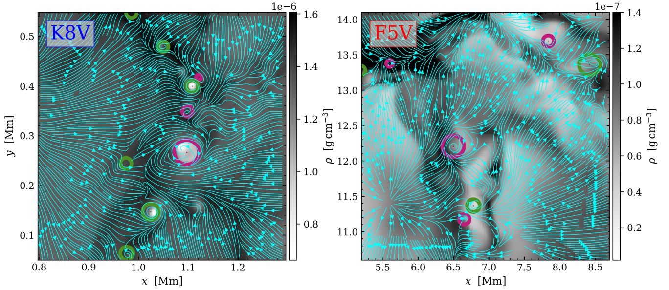
Fig. A.2. Identified swirls in the areas depicted in blue in Fig. A.1 for the K8V and F5V models. Pink disks represent clockwise swirls, green counter-clockwise swirls. The horizontal component of the velocity field is represented by blue instantaneous streamlines.
