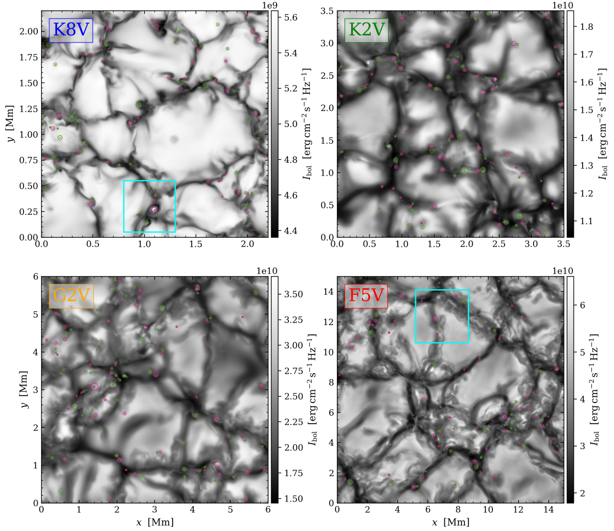
Fig. 1. Emerging bolometric intensity, I_{\text{bol}} , for the K8V, K2V, G2V, and F5V models during the kinematic phase. Clockwise and counterclockwise vortices in the horizontal plane at z = 0 identified by the SWIRL algorithm are indicated by pink and green disks, respectively. The blue squares in the K8V and F5V panels mark the boundaries of the zoomed plots shown in Fig. 2.
