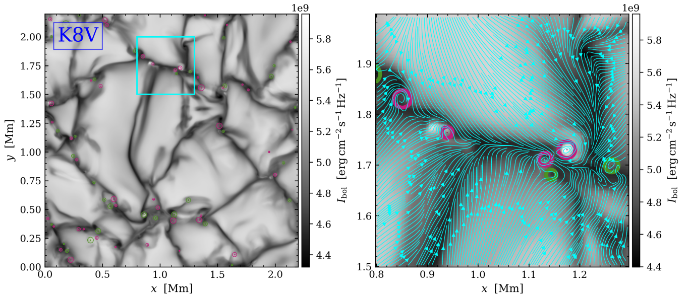
Fig. B.1. Emerging bolometric intensity, I_{\text{bol}} , for the K8V stellar model during the saturation phase of the SSD. Clockwise and counterclockwise vortices in the horizontal plane at z = 0 km identified by the SWIRL algorithm are indicated by pink and green disks, respectively. The blue square in the left panel marks the boundaries of the zoomed region shown in the right panel, where the horizontal component of the velocity field at z = 0 km is represented by blue instantaneous streamlines.
