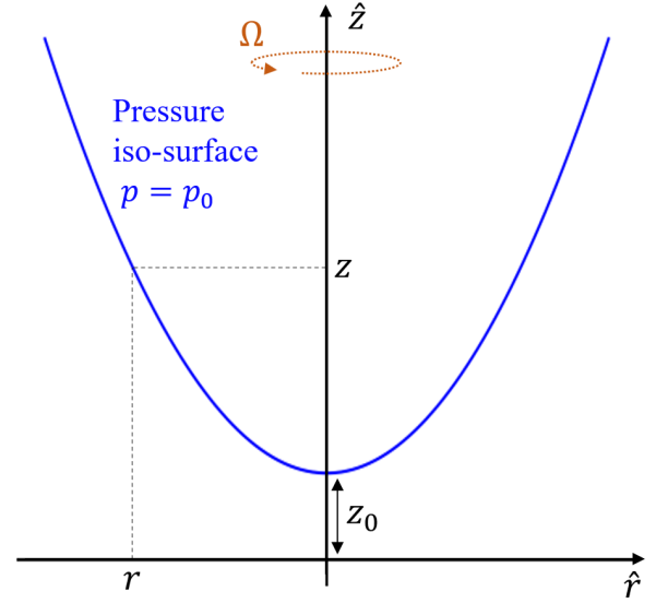
Fig. 8. Two-dimensional representation of an axially symmetric flow rotating at angular velocity \Omega . The surface of constant pressure p = p_0 is shown, where p_0 is the pressure at (r, z) = (0, z_0) .
