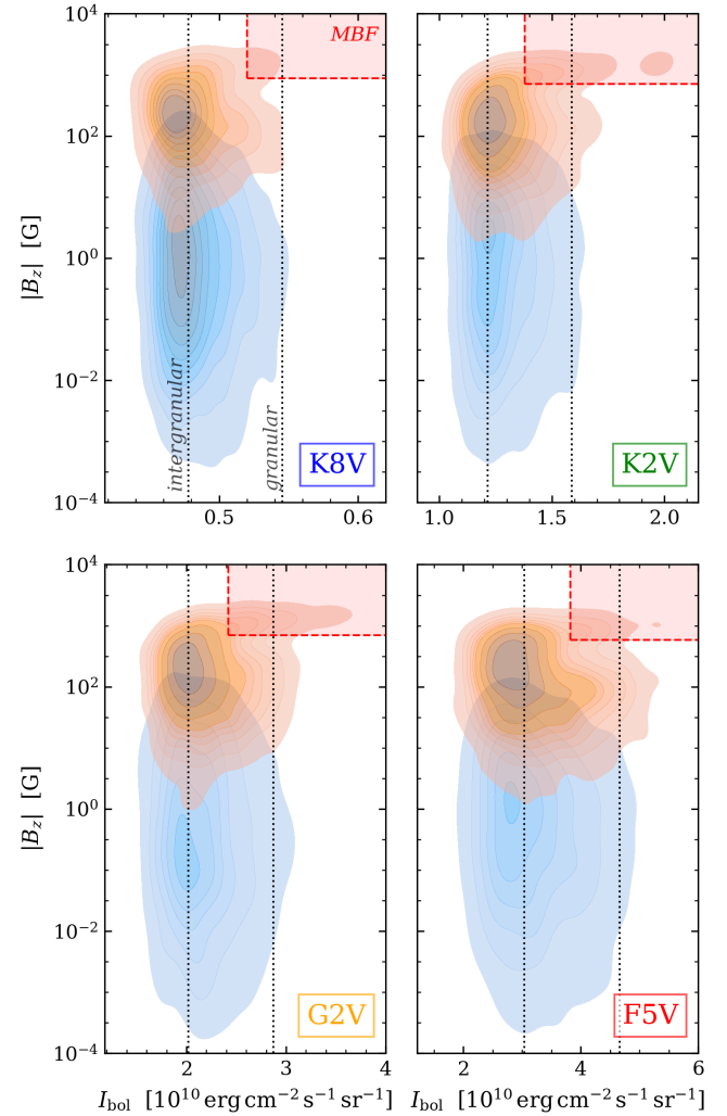
Fig. 3. Bivariate distribution of the bolometric intensity I_{\text{bol}} and the absolute vertical magnetic field |B_z| in the center of the swirls identified on the surface layer at z = 0 km of the four stellar models. The distributions during the kinematic and saturation phases are shown in blue and orange, respectively. The vertical black dotted lines indicate the mean bolometric intensity in the intergranular (lower value) and granular (higher value) regions. The red shaded area indicates the identification range of magnetic bright feature (MBF) as defined by Riva et al. (2024).
