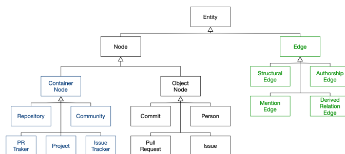
Fig. 1. The Model of a Software Project
